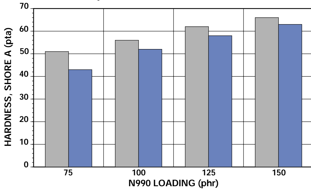
Figure 1b Effects of N990 in Butyl Rubber* – hardness
