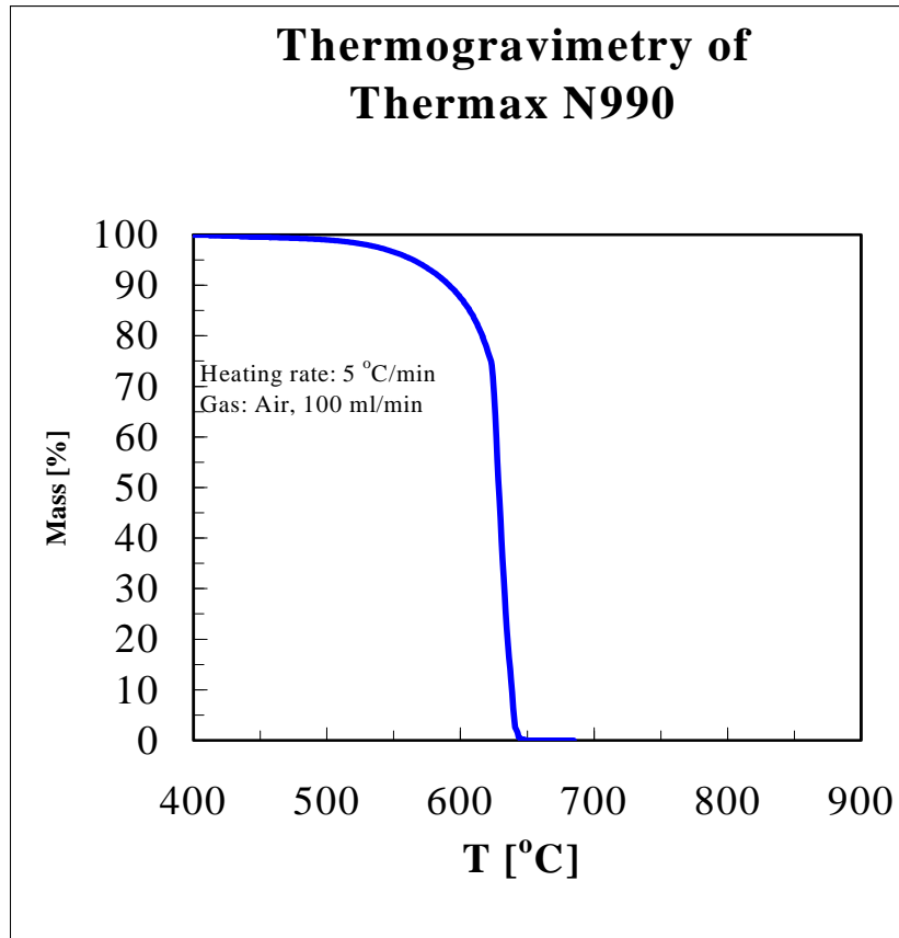
Figure 2: TGA of Thermax®
